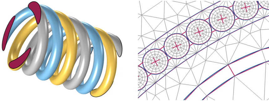
Figure 4: The cross-sectional cut of a helix (left), and the truncation of circles (right).
