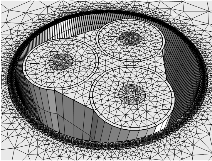
Figure 2: The swept mesh in the phases, screens, and armor. The void region between the screens and the armor will use a free tetrahedral mesh (not shown in this image).
