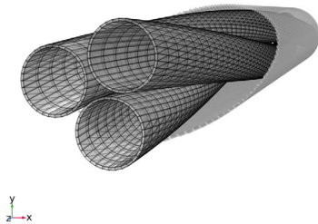
Mesh quality, poor quality elements
